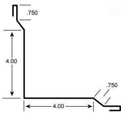
14. Inside Corner
