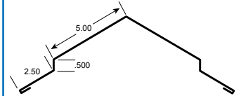
10. Ridge Cap
