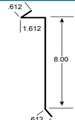
Reglet Flashing (not shown)
