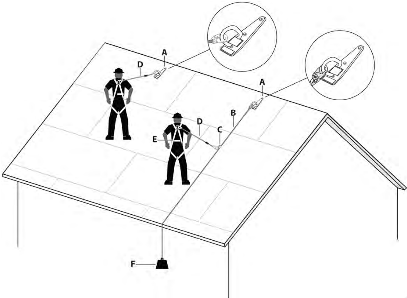
Figure 2B: Roof Anchors for Restraint Applications
