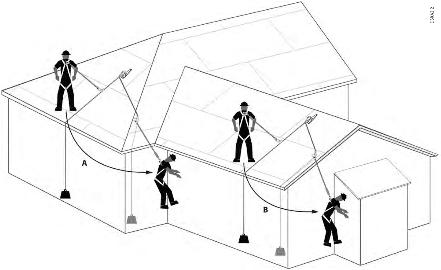
Figure 3: Typical Swing Fall Hazards from Roofs
