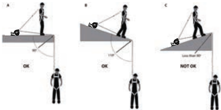
Figure 5 - Leading Edge Angle of Lifeline Redirect
