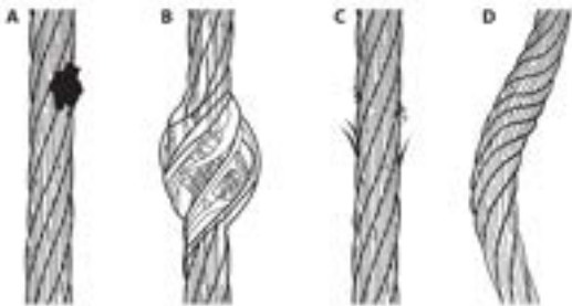
Figure 9: Inspection of Cable
