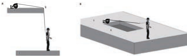
Figure 7 - Incorrect Use of Leading Edge SRD
