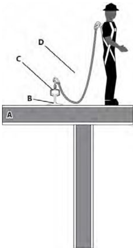
Fig. 4: Swing Fall with Foot-Level Tie-Off
