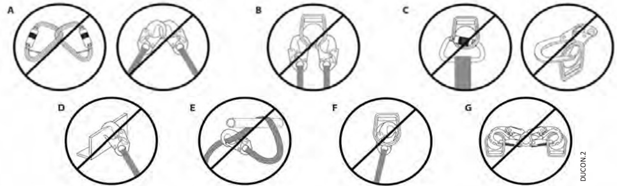
Fig. 9 - Incorrect Connections
