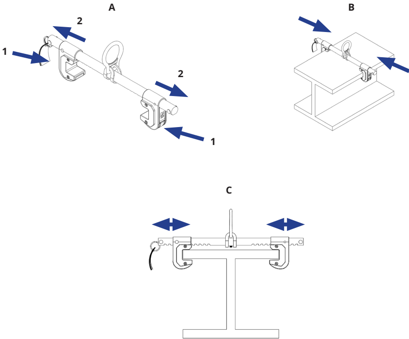
Figure 4 - Installation Instructions
